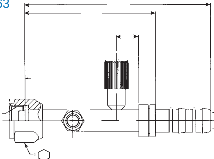
Straight – Female O-ring (Short Pilot), with R134a Low Side Port and Female Switch Connection, (1/8-27 Thread)
