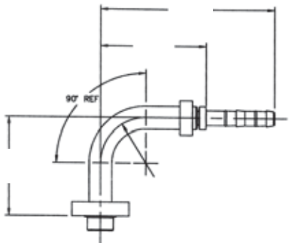
90° Pad Style Connection (Volvo) (Pad Orientation 90°)
