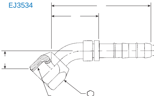
45° Female JIC 37° Flare
