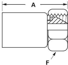
Air Brake Swivel
