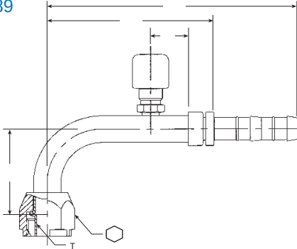
90° Female O-ring (Long Pilot) with Charge Port (7/16-20 thd)
