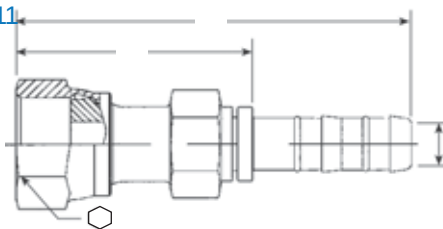
Straight - ORS Female Swivel Metric Hex Nut
