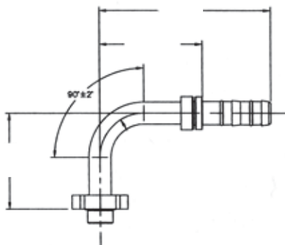
90° Pad Style Connection (Volvo)
