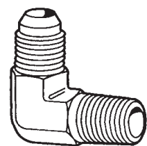
Male British Standard Tapered Pipe to Male SAE 37° SAE 90° Elbow
