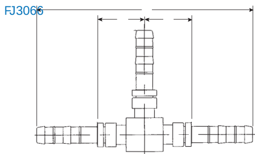
"T" Splicer - 3 Hose Connector
