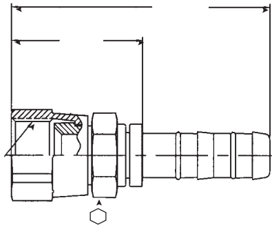
Straight – Female 37° Flares
