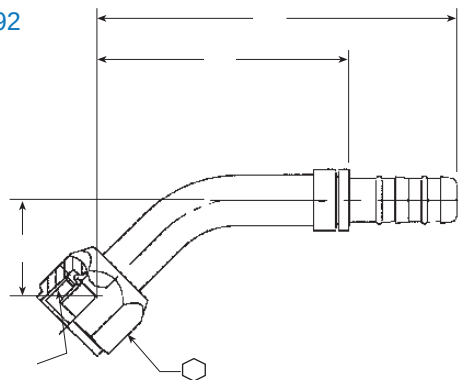
45° Female O-ring (long pilot, metric thread)
