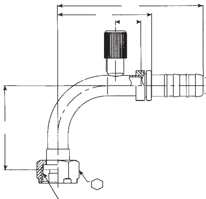
90° Female Rotalok with R134a Low Side Port
