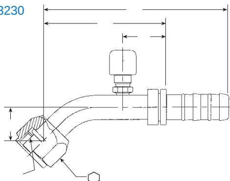
45° Female O-ring (Long Pilot) with Switch Port (7/16-20 thd)
