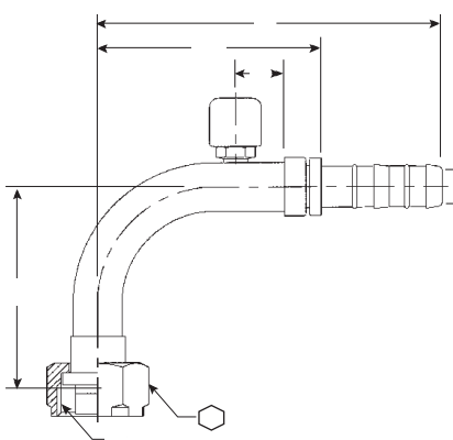
90° Female Rotalok with Switch Port (7/16-20 Thread)
