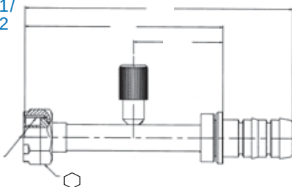
Female Rotalok with R134 Port
