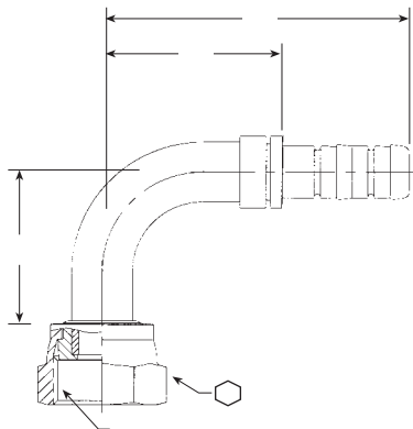
90° ORS Female Swivel (Long Drop)
