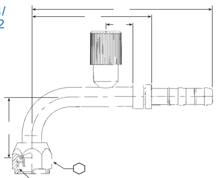
90° Female O-ring (Short Pilot) with R134a High Side Port
