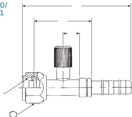
Straight – Female O-ring (Long Pilot) with R134a High Side Port (Metric Thread)
