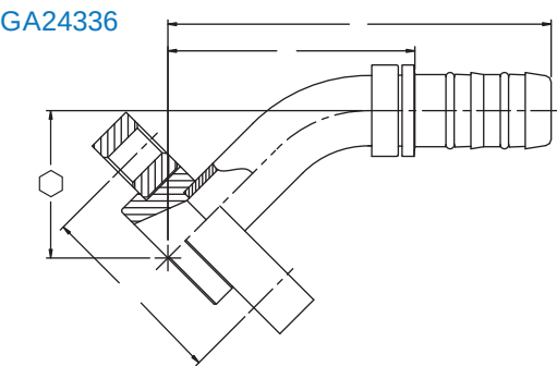
45° Bock Compressor Fitting
