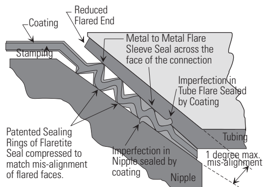
Flaretite Seal Joint Section of Applied Seal
